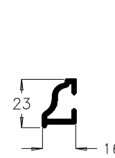
Weather bar P10149
