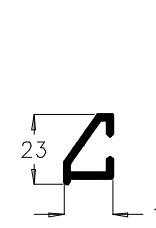
Weather bar P10317
